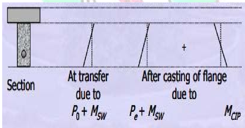
Figure 9-1.3 Stress profiles for the precast web
