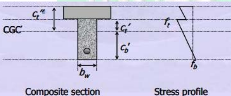
Figure 9-1.7 Stress profile for the composite section
