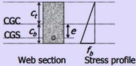
Figure 9-1.6 Stress profile for maximum eccentricity of CGS
