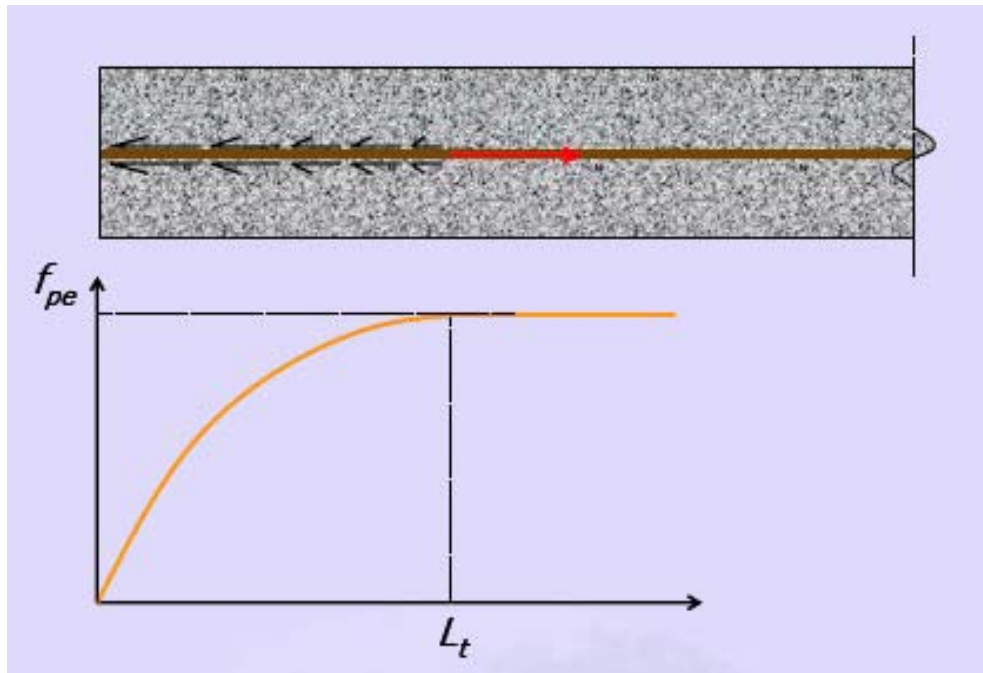
Figure :Variation of prestress in tendon along transmission length
