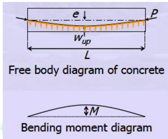
Simply supported beam with parabolic tendon
